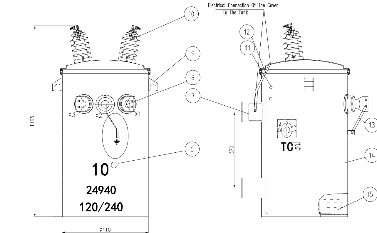
HV BUSHING TERMINAL
