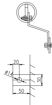
Low-Voltage Grounding Strap Connection
