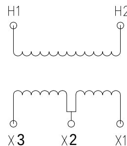
HV BUSHING TERMINAL
